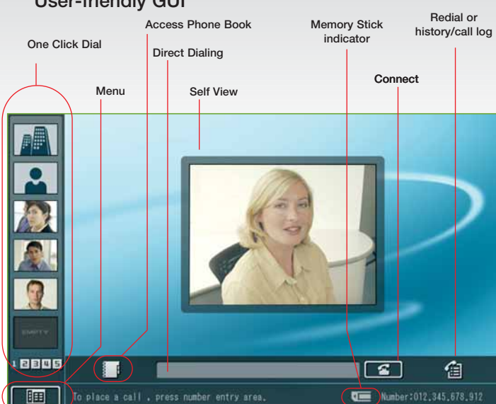
STARTUP WINDOW
